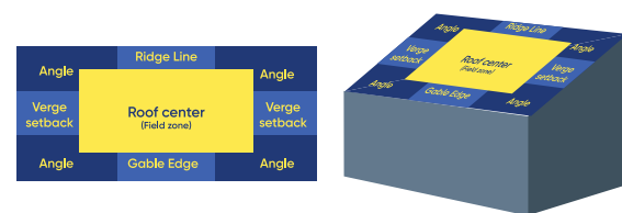
MONO-PITCH ROOF
