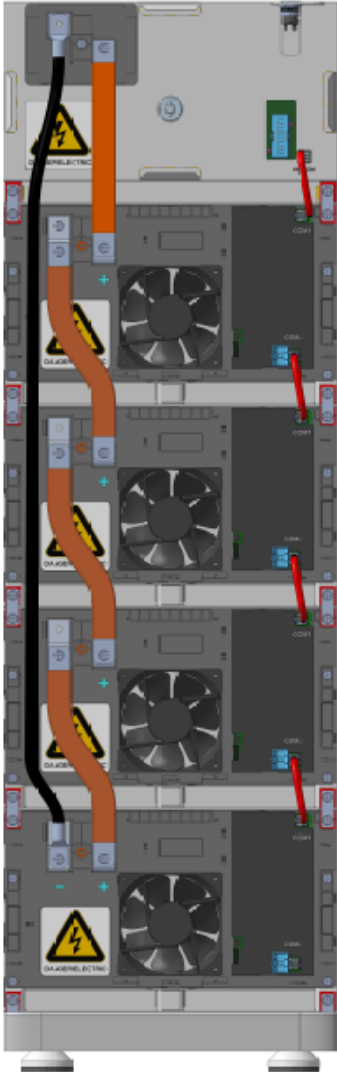
4 packs-64.28kWh
